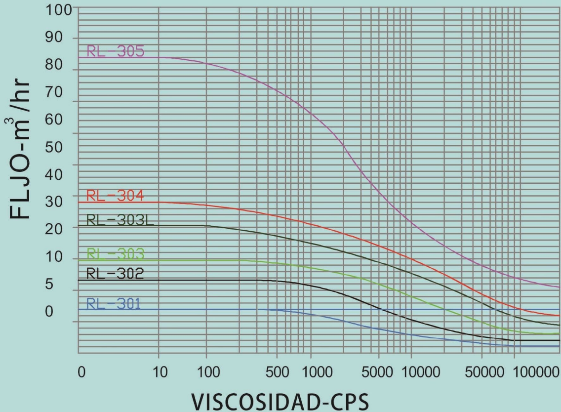
光星Rotary Lobe Pumps性能曲線圖 RL-3 performance curve
